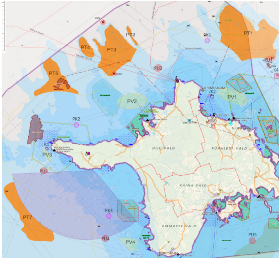
Figure 2.10. An extract from the County plan of the marine area bordering Hiiu County (not adopted as of October 2015). Orange areas mark the potential areas for building offshore wind parks.
